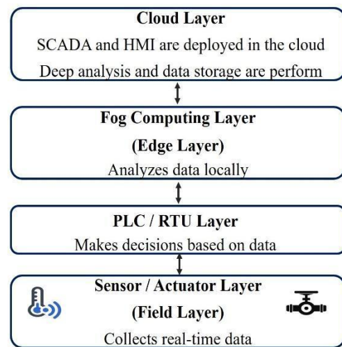
Fog-based SCADA system architecture
